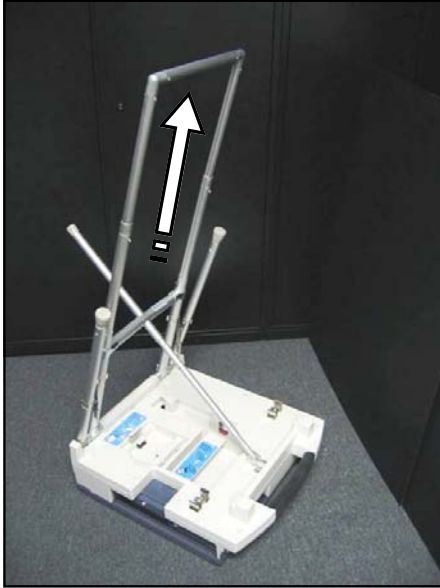
STEP TWO — Pull the inside leg all the way up, until it clicks into place. You will hear two clicks.
